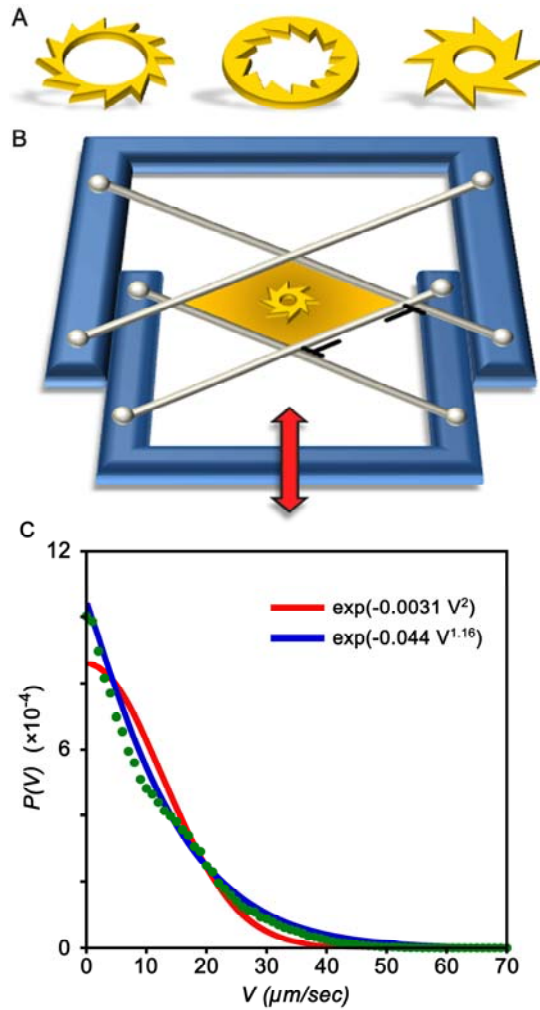
Figure 1. Experimental design. (A) Shapes of some types of gears used in this study (B) Scheme of the experimental setup. The film is suspended between four wires attached to a moveable frame. Film thickness is controlled by the linear motion of the frame (indicated by the red arrow). The experimental apparatus is placed in a transparent chamber with controlled atmosphere and mounted on the moving stage of inverted microscope. (C) Velocity distribution function P(V) for small fluorescent tracers ( 2.5 \mu\text{m} polystyrene microspheres, Spherotech, Inc.) advected by Bacillus subtilis bacteria in the regime of collective swimming at concentration 2 \times 10^{10} \text{ cm}^{-3} . Corresponding root-mean-square (rms) velocity, V_{\text{rms}} , of the tracers is about 13 \mu\text{m}/\text{sec} . Red line gives the best fit to the Gaussian law, and blue line is a stretched exponential fit with the exponent 1.16.
